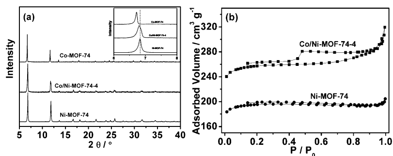
Figure 1. (a) XRD patterns of the as-prepared Ni-MOF-74, Co/Ni-MOF-74-4, and Co-MOF-74 (inset shows enlarged regions of the XRD patterns); (b) N_2 adsorption/desorption isotherms of prepared Ni-MOF-74 and Co/Ni-MOF-74-4 (77 K).
